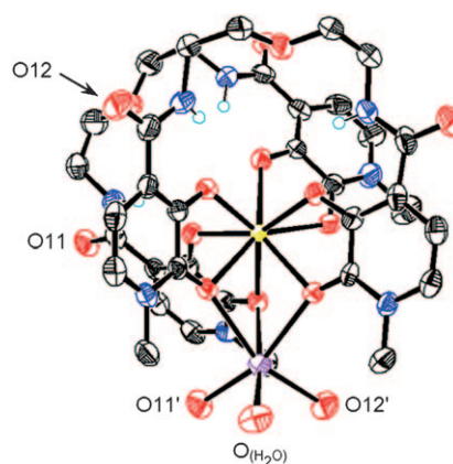
Figure 1. A view of the X-ray crystal structure for \text{Na}[\text{Ho}(\text{5LIO-3,2-hopo})_2] . Thermal ellipsoids of non-hydrogen atoms are drawn at the 50 % probability level (black C, red O, blue N, yellow Ho, purple Na). Cocrystallized DMF and selected hydrogen atoms have been omitted for clarity.
